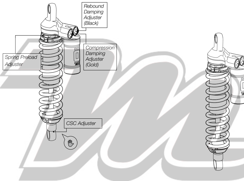
Öhlins Shock Absorber TTX44 BM984
